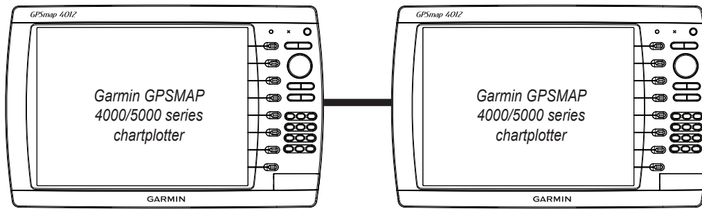
Marine Network with Two Chartplotters
