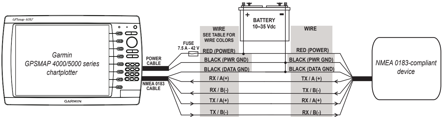
Wiring to a Standard NMEA 0183-compliant Device with 2-way Communication
