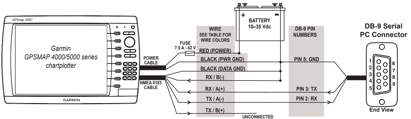
Wiring to a DB-9 Serial PC Connector
